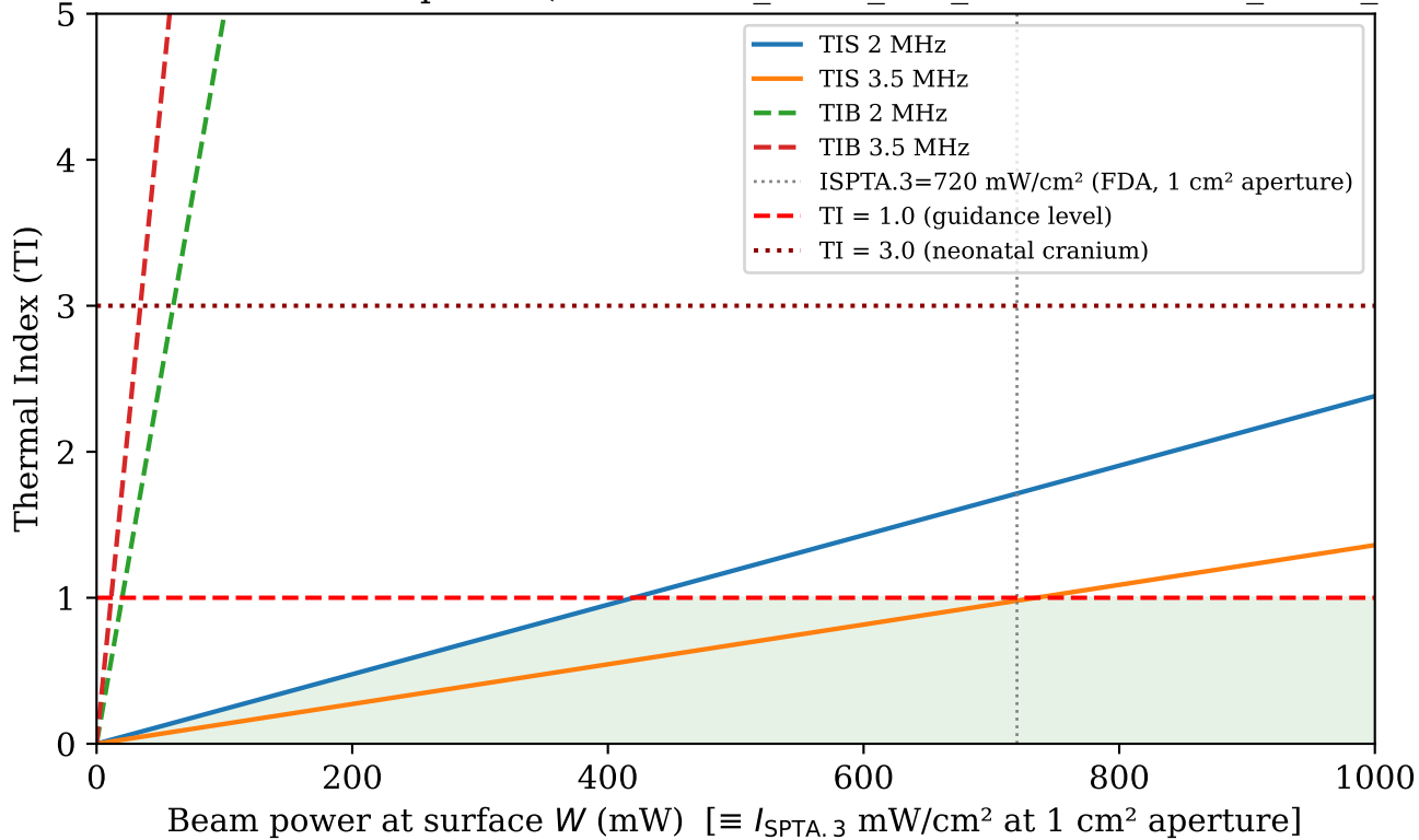
Thermal Index vs beam power (kw.thermal_index_soft_tissue / thermal_index_bone)
