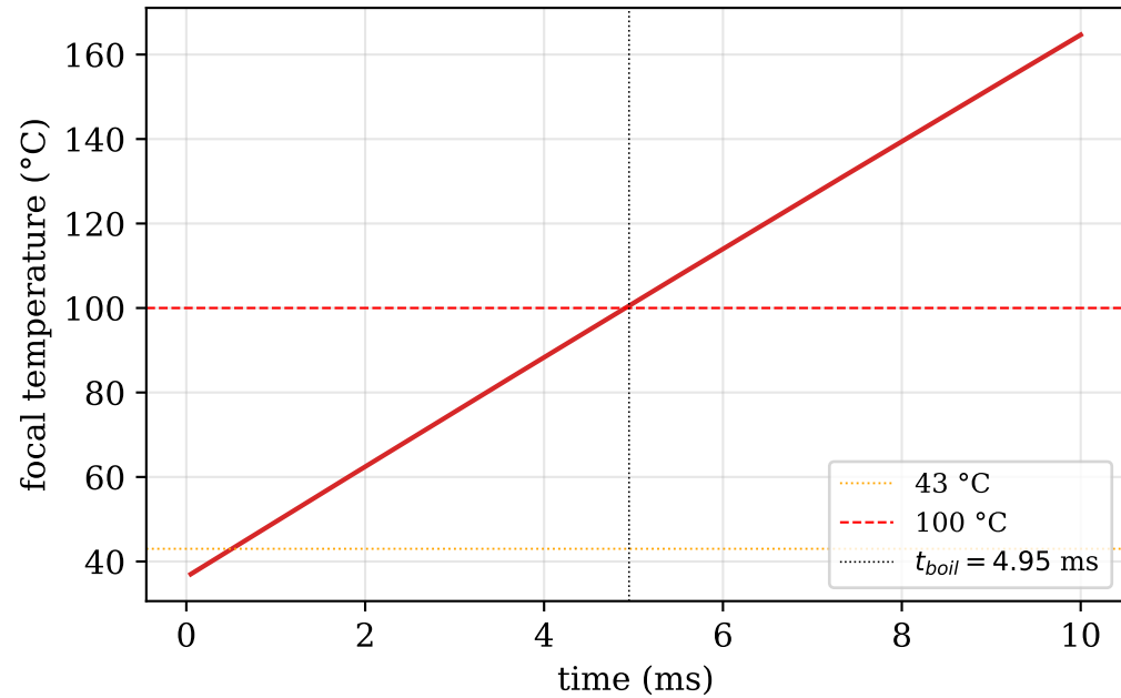
Millisecond, peak T = 165 °C (kwavers ThermalDiffusionSolver + Pennes bioheat)
