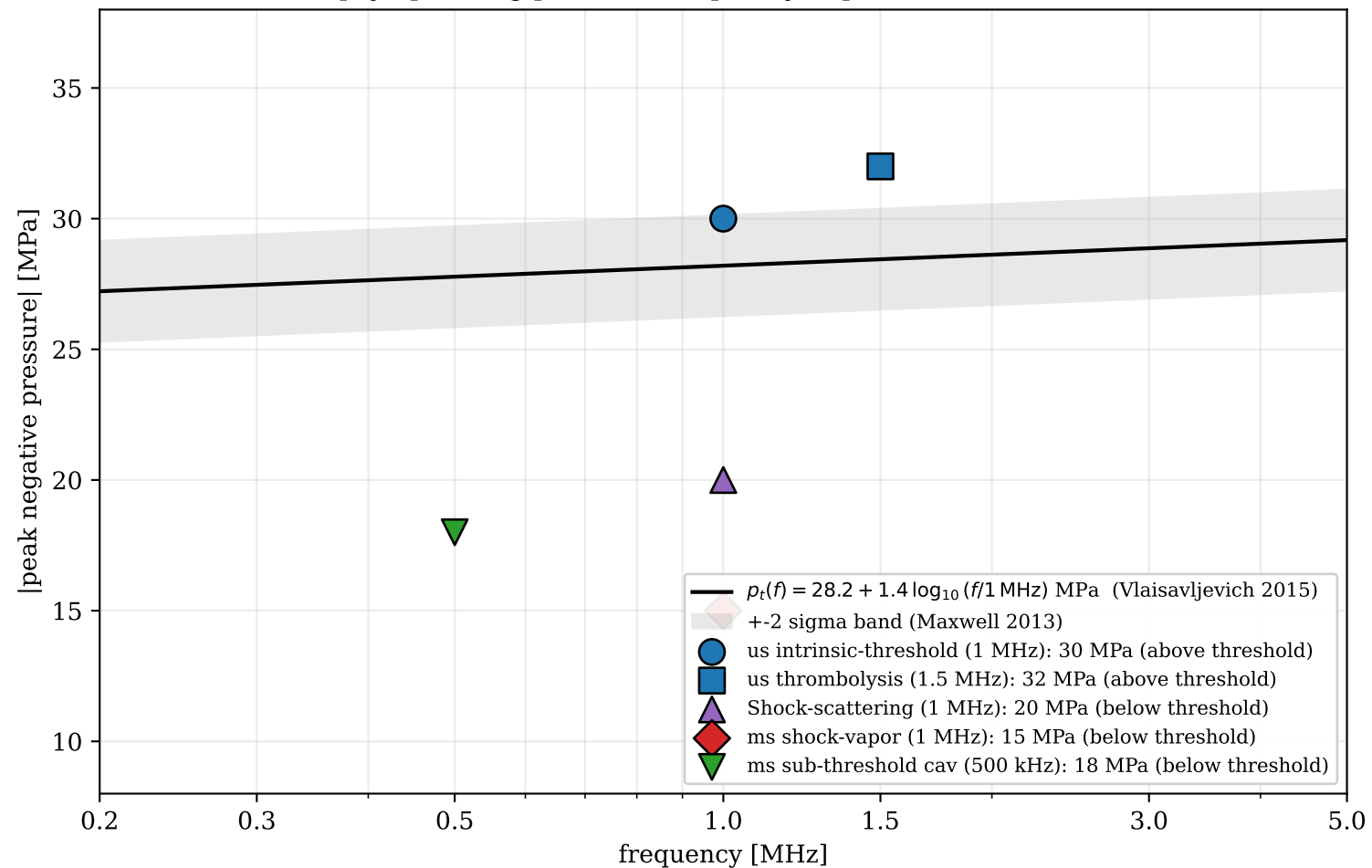
Histotripsy operating points vs frequency-dependent intrinsic threshold
