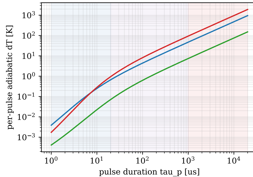
Single-pulse focal temperature rise
