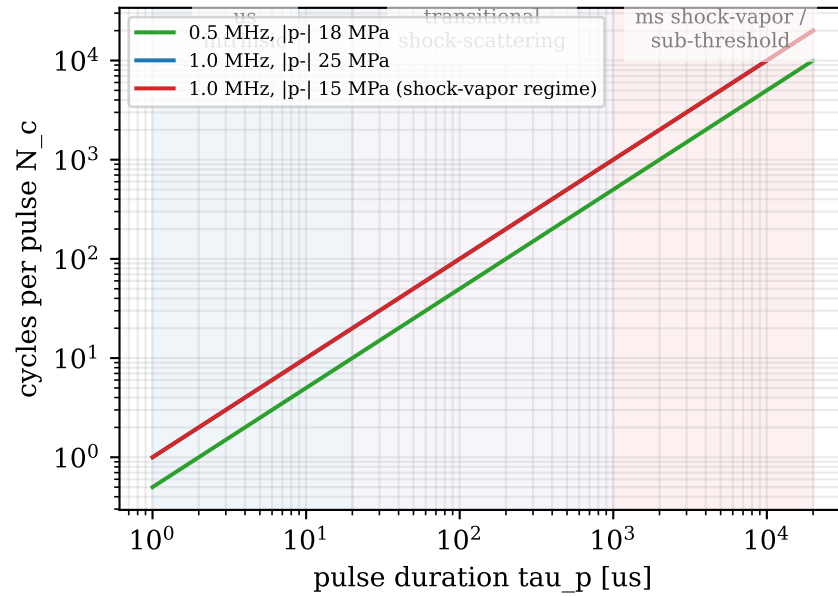
Pulse cycle count
