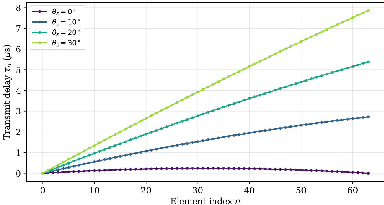
Linear-Array Steering Delay Law (Eq. 4.11) 64 elements, d = \lambda/2 , focus on natural-focus arc N = 197 mm
