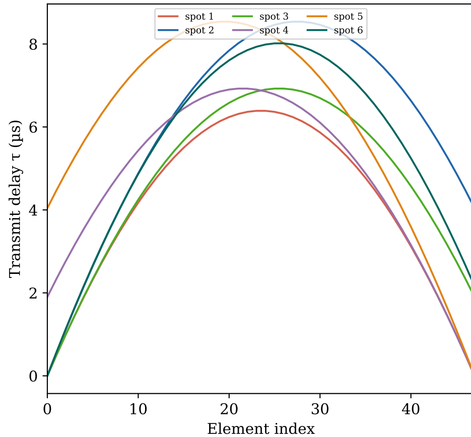
(B) Delay-to-target laws \tau = (\max r - r) / c per sub-spot
