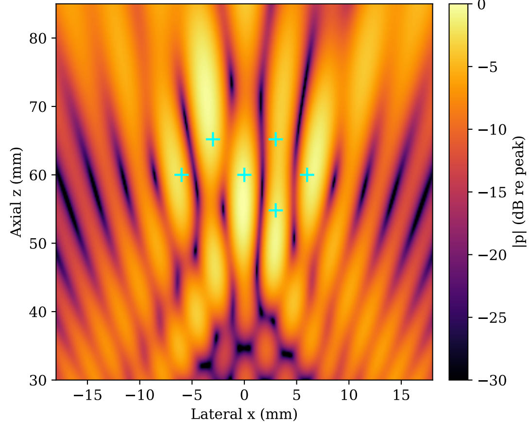
(C) Simultaneous multi-focus field phase-conjugation synthesis (dB re peak)
