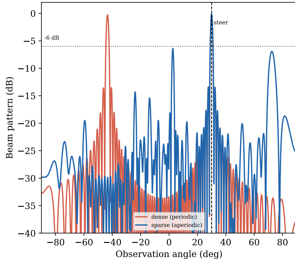
(B) Beam pattern steered to 30 deg dense grating lobe vs sparse pedestal
