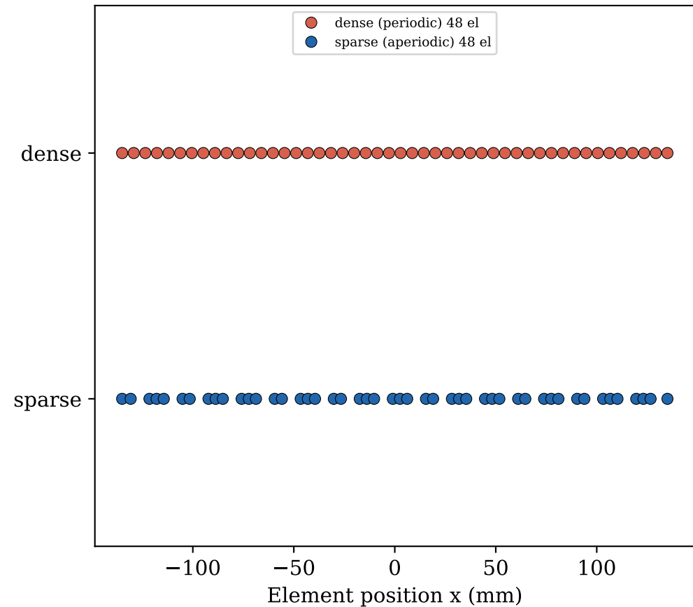
(A) Same 48 elements, same 270 mm aperture pitch / lambda = 0.84 @ 220 kHz
