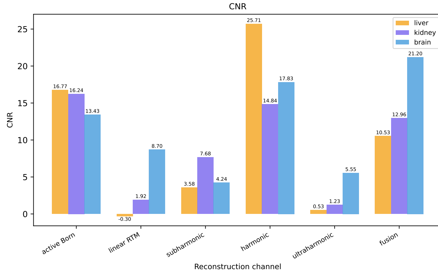
Reconstruction fidelity — Dice (equal-area), CNR, and passive operator-vs-PAM
