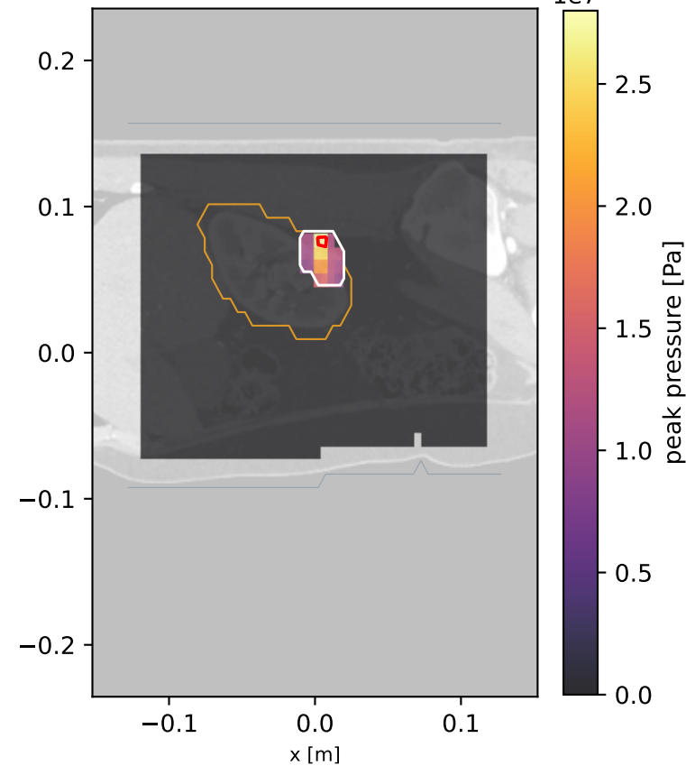
Focused-US treatment-support peak = 28.00 MPa red: intrinsic-threshold cavitation isoline (26 MPa)
