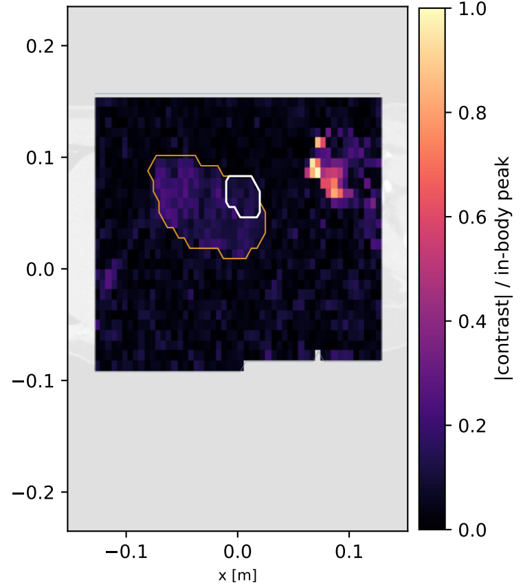
Reconstructed image (linearised Born, single-pass H^1 -Tikhonov) in-body peak = 0.246 (a.u.), multi-frequency imaging transmit, same aperture
