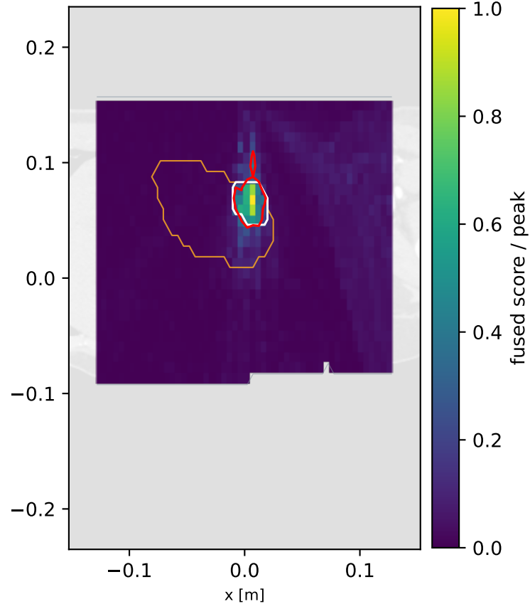
Fused lesion-localization image peak = 1, Dice = 0.82, CNR = 13.0
