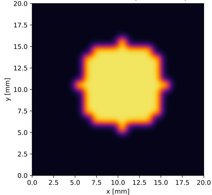
True shear modulus \mu (3x stiff lesion)
