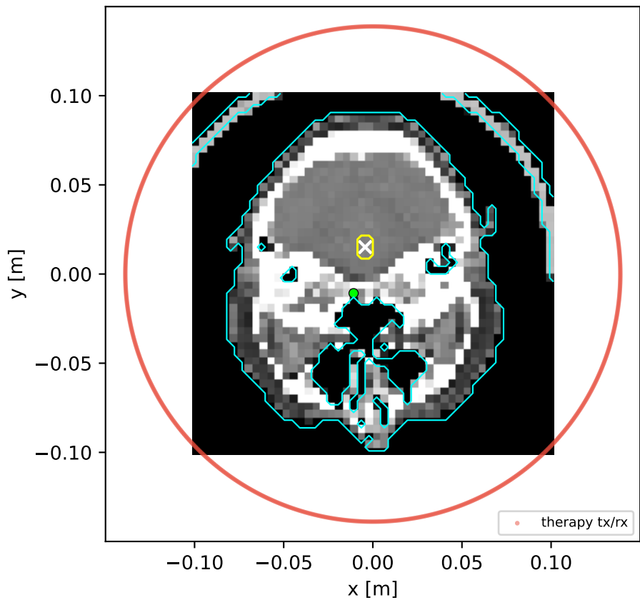
brain: INSIGHTEC-like helmet 1024 elements, helmet clearance 15.0 mm
