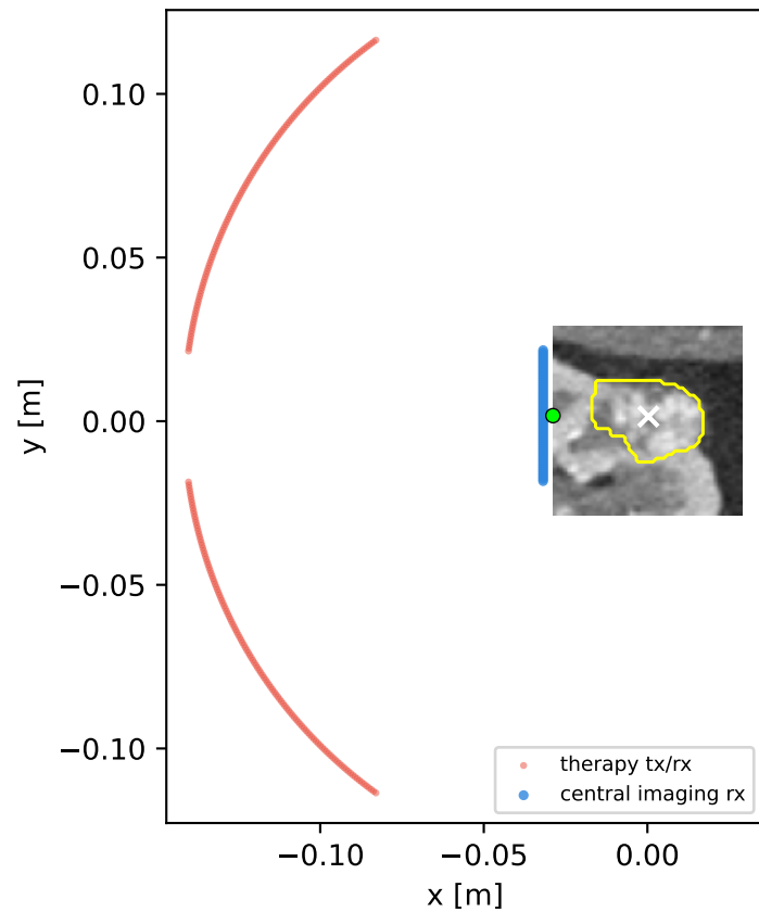
kidney: HistoSonics-like skin arc 256 elements, skin gap 3.0 mm
