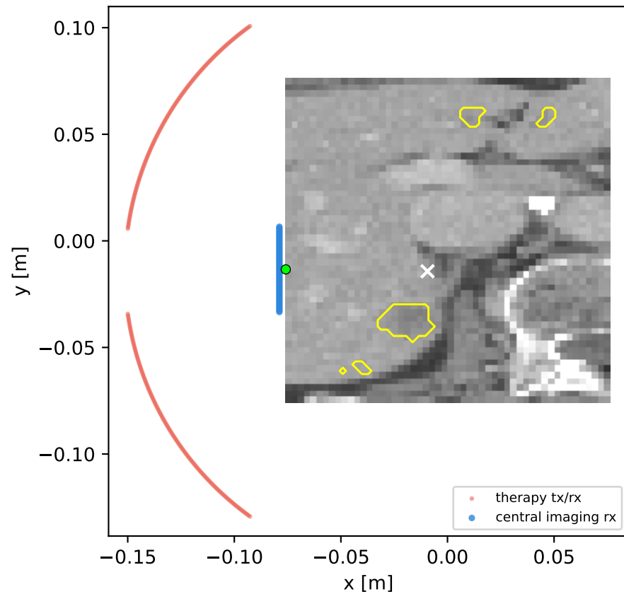
liver: HistoSonics-like skin arc 256 elements, skin gap 3.0 mm
