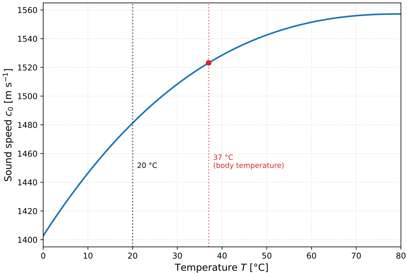
Figure 1.5 — Sound speed in water vs temperature c(T) = 1402.7 + 4.83T - 0.0487T^2 + 1.47 \times 10^{-4}T^3 (Del Grosso-Mader)
