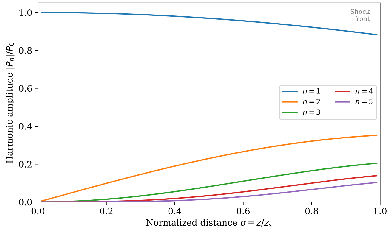
Fubini Harmonic Spectrum — Pre-shock ( \sigma < 1 )
