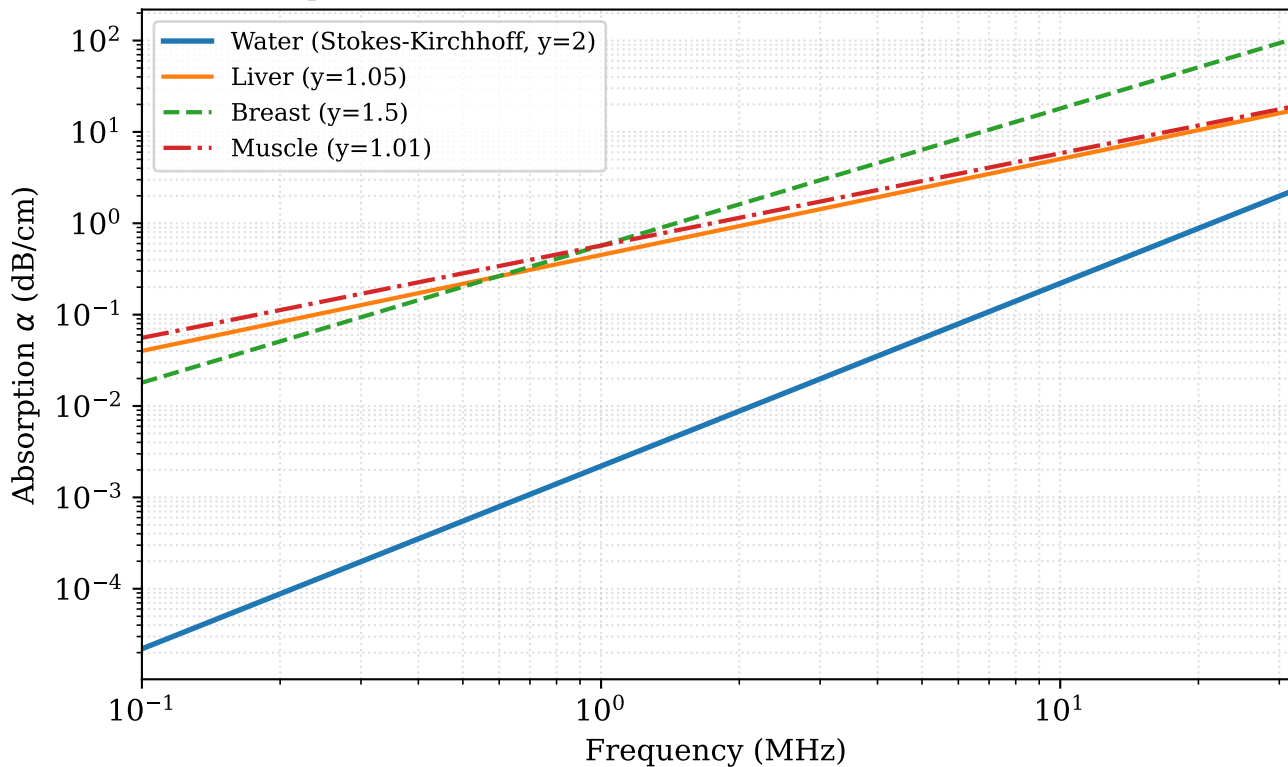
Absorption Coefficient — Classical vs Power-Law (Duck 1990)
