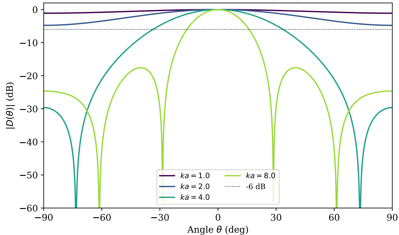
Baffled Circular Piston Directivity (Eq. 4.3)
