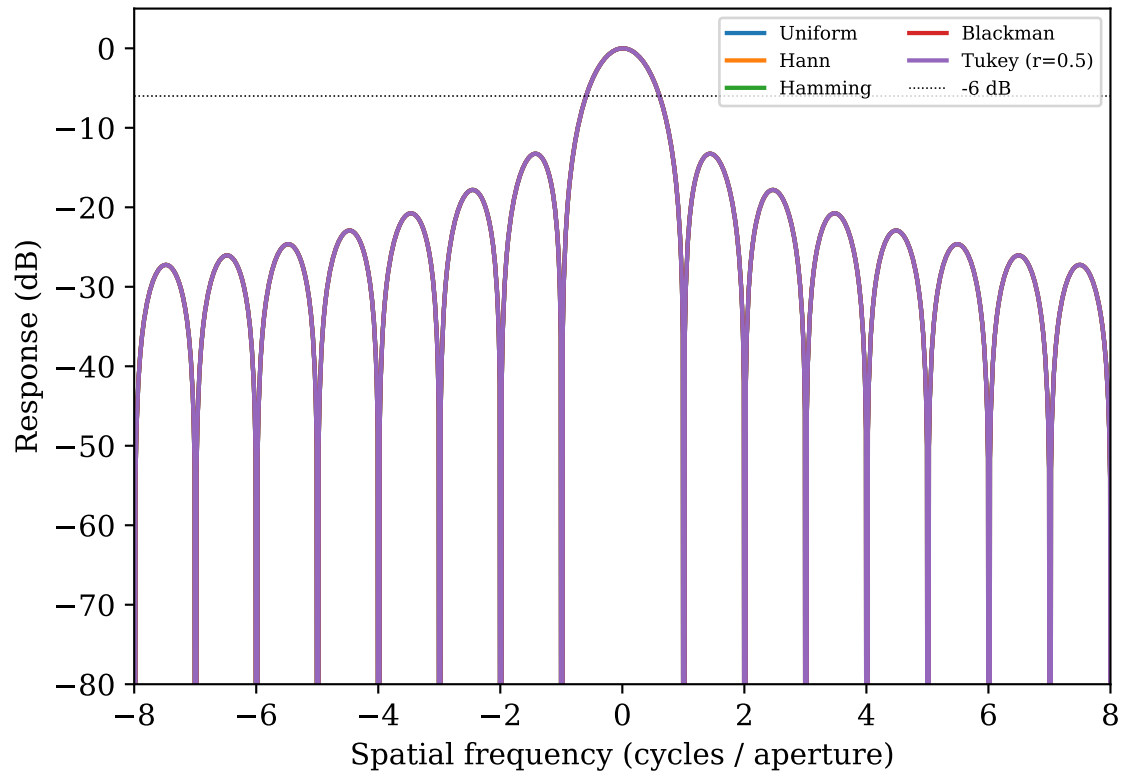
Frequency Response (sidelobe envelope)
