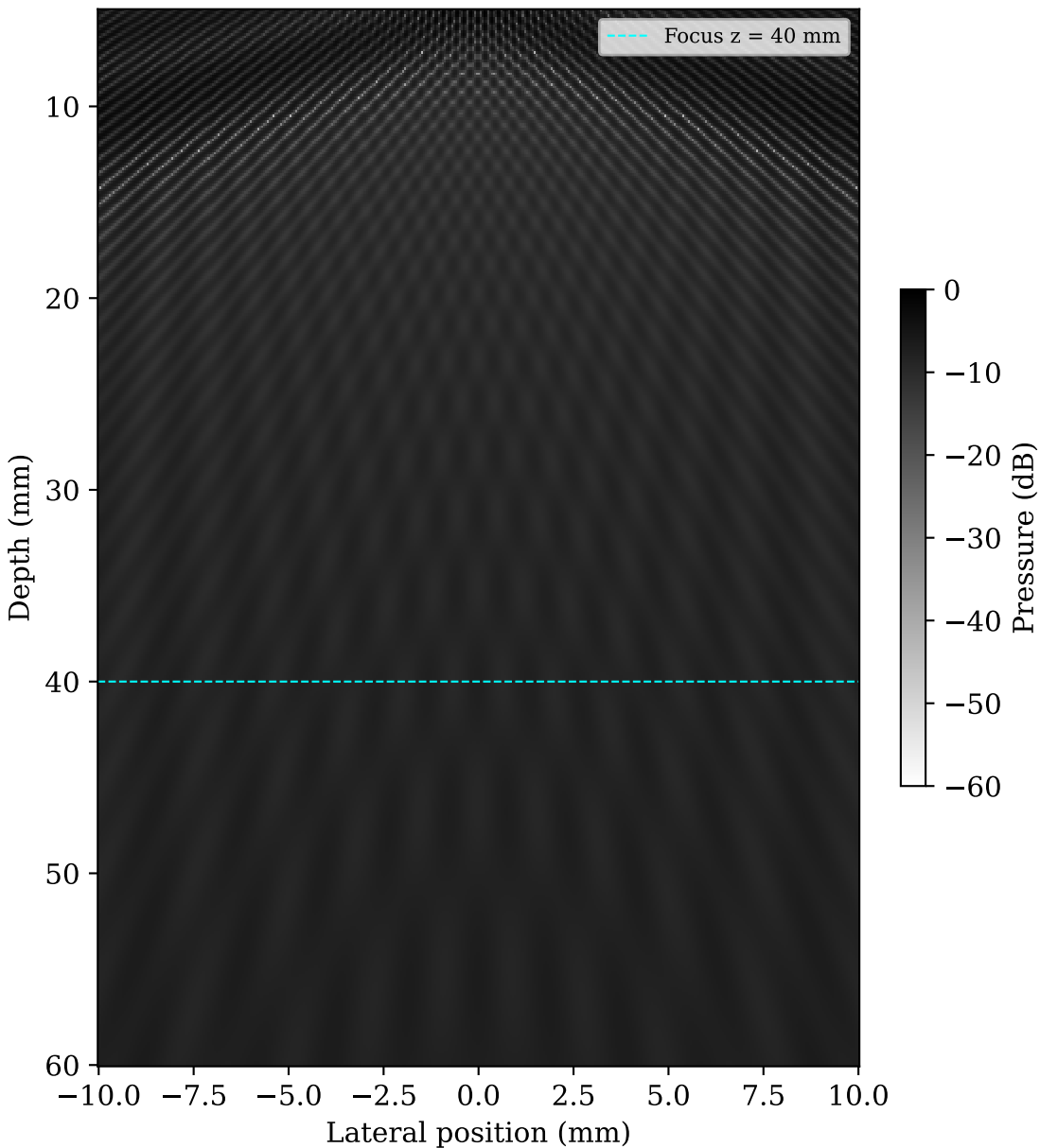
2-D Beam Pattern - 64-element linear array Hann apodization, f_0 = 5 MHz, d = 0.3 mm
