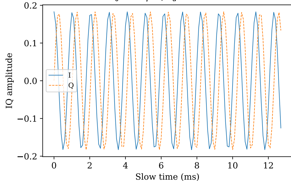
Slow-time IQ — contrast agent R_0 = 1.5\ \mu\text{m} , P_a = 100\ \text{kPa}
