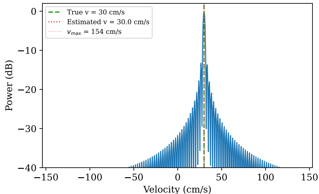
Contrast-Agent Doppler Spectrum — f_0 = 5\ \text{MHz} , \alpha = 60.0^\circ RP amplitude: A_{\text{bubble}} = 0.183 ; Doppler shift from pykwavers
