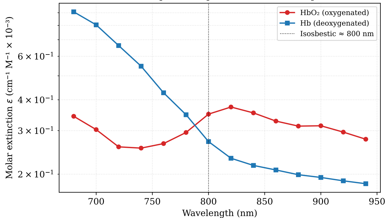
Hemoglobin Absorption Spectra (Prahl 1999) Used for PA spectroscopic sO 2 estimation (Eq. 5.20)
