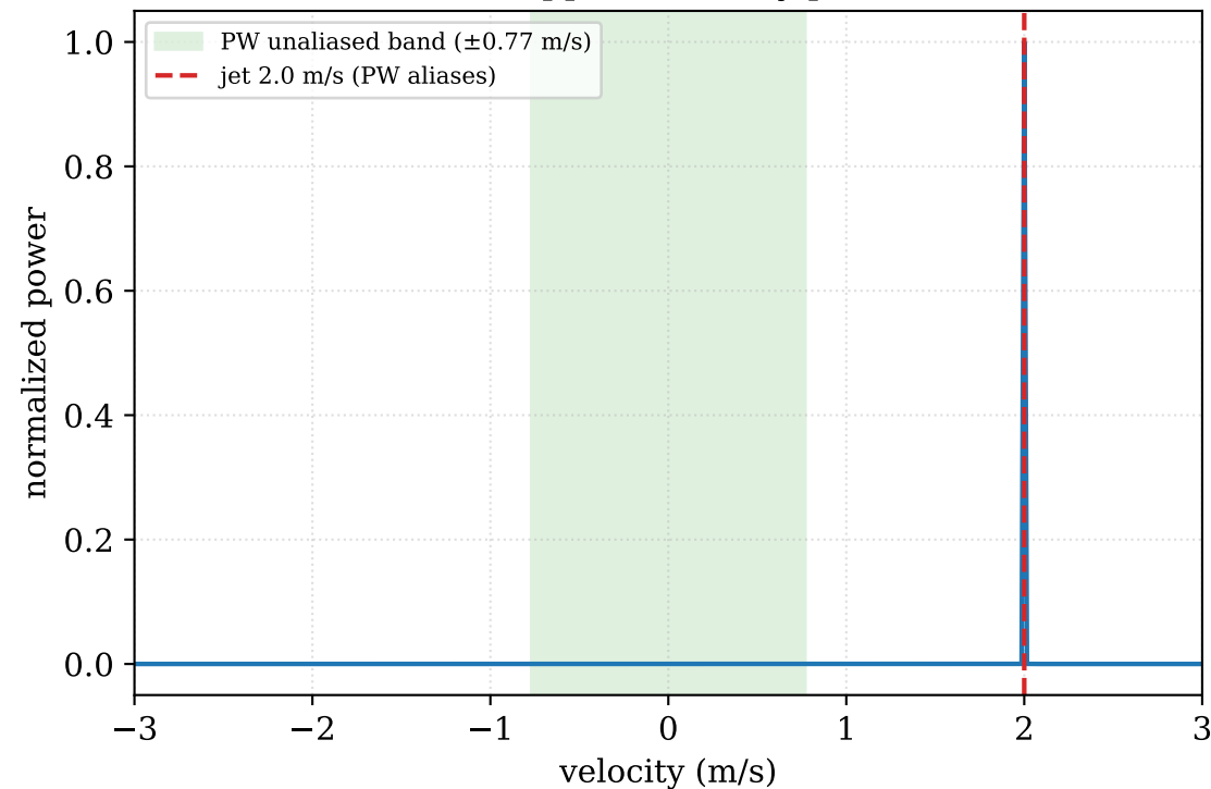
(a) CW Doppler — no Nyquist limit
