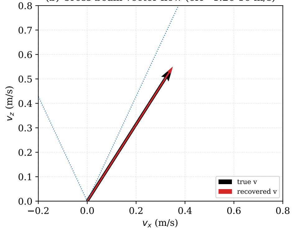
(b) Cross-beam vector flow (err= 1.2\text{e-}16 m/s)
