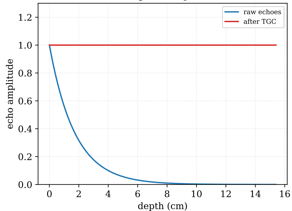
(a) Time-gain compensation
