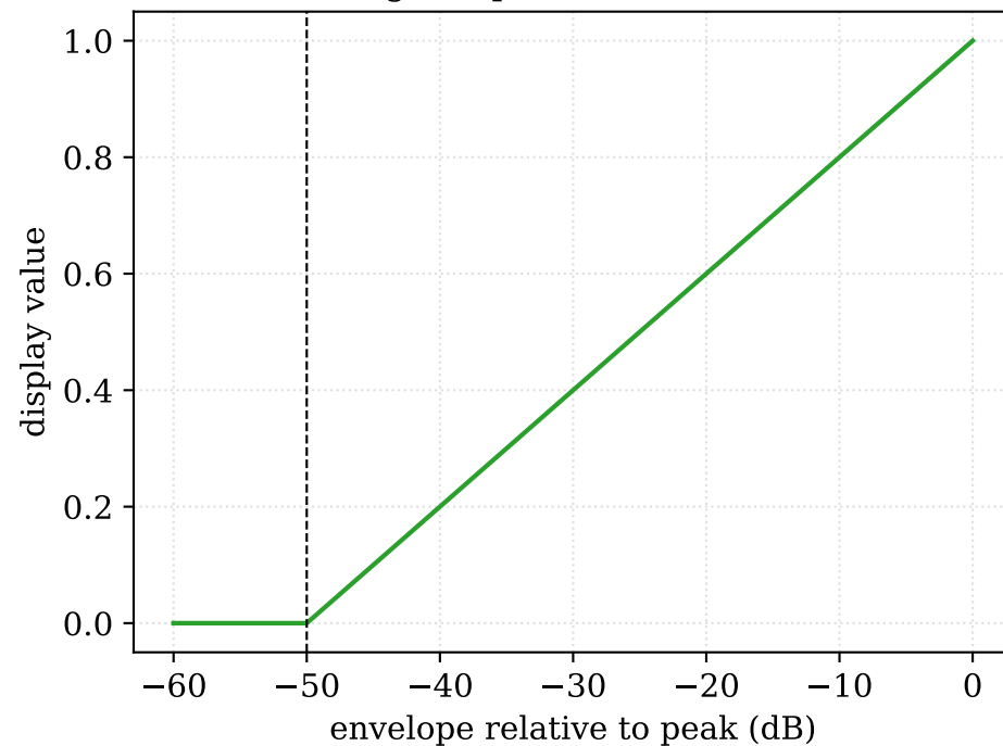
(b) Log compression (DR=50 dB)
