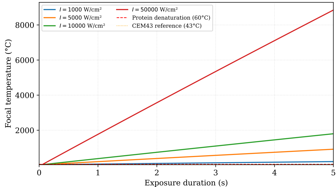
Focal Temperature Rise — Liver, f_0 = 1 MHz (Eq. 6.4, Pennes bioheat: diffusion + perfusion; kwavers ThermalDiffusionSolver)
