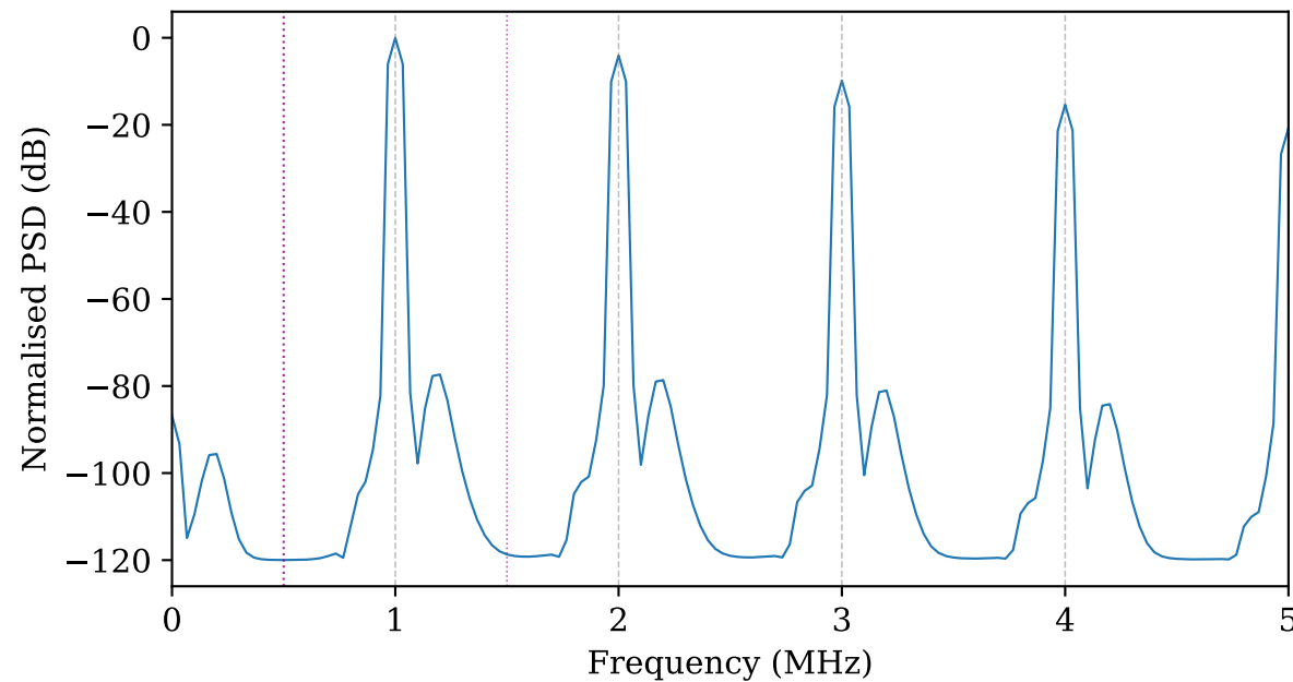
Stable Cavitation (SC) P_a = 50\text{ kPa} , MI = 0.050
