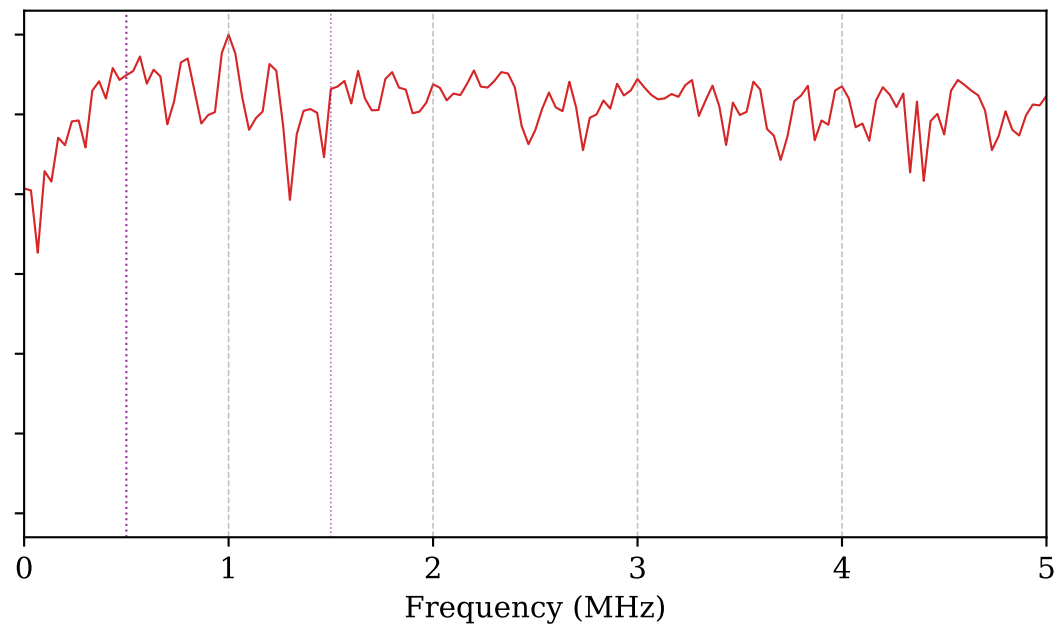
Inertial Cavitation (IC) P_a = 400\text{ kPa} , MI = 0.400
