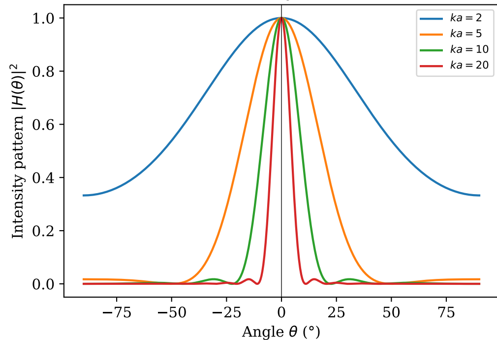
Piston directivity (linear scale)
