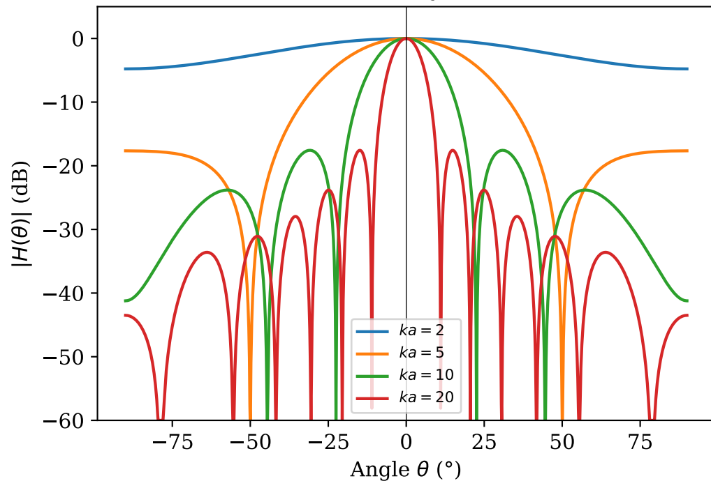
Piston directivity (dB scale)
