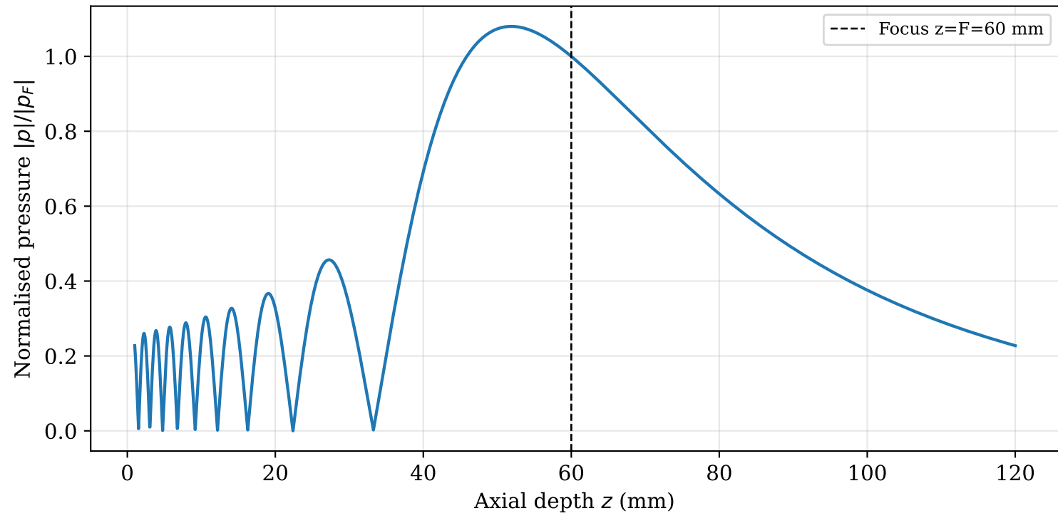
Focused bowl on-axis pressure F = 60 mm, a = 15 mm, f = 1 MHz, c = 1500 m/s
