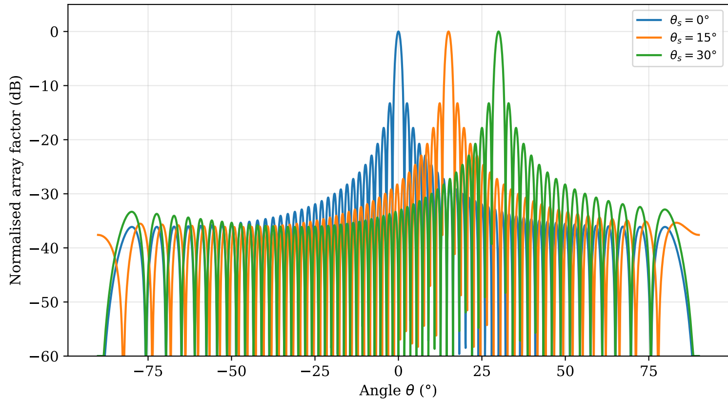
Linear phased array beam pattern N = 64 , d = 0.3 mm, f = 2.5 MHz
