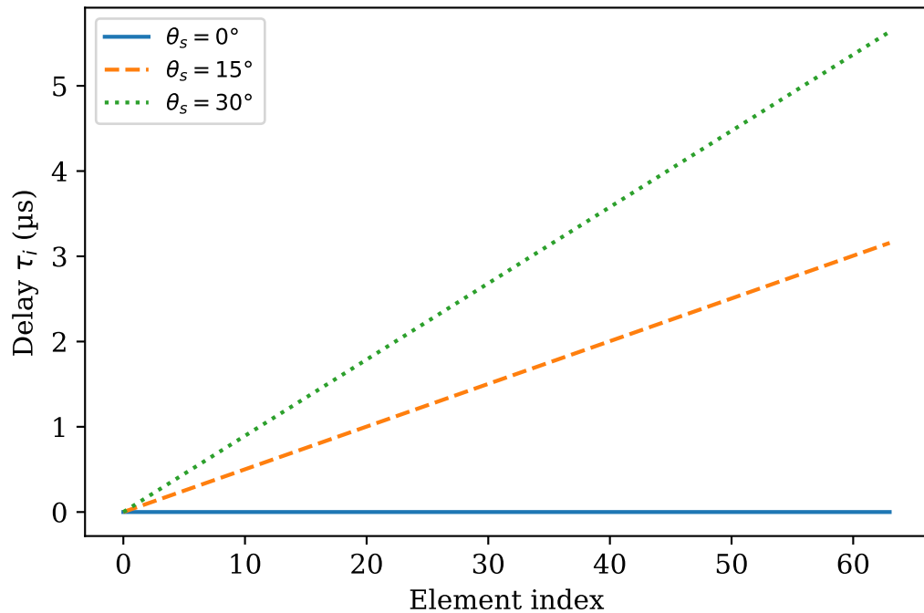
Steering delay law (far-field focus)
