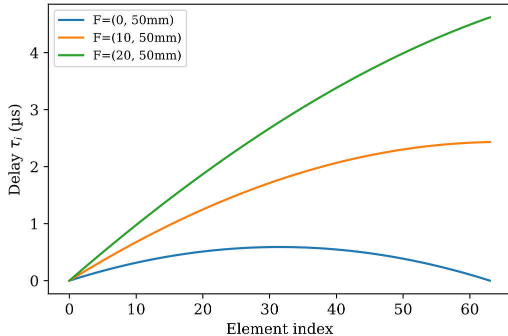
Focusing delay law (near-field)
