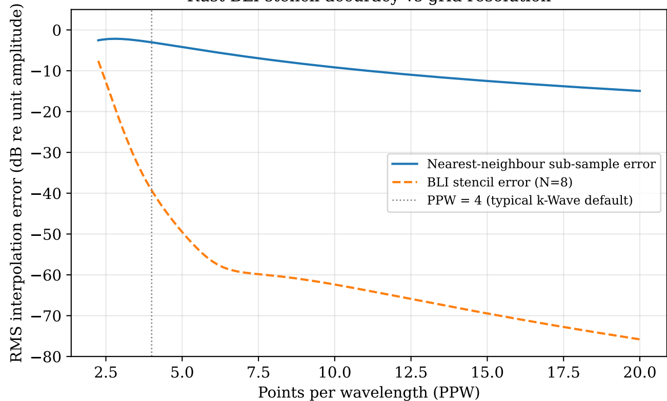
Rust BLI stencil accuracy vs grid resolution
