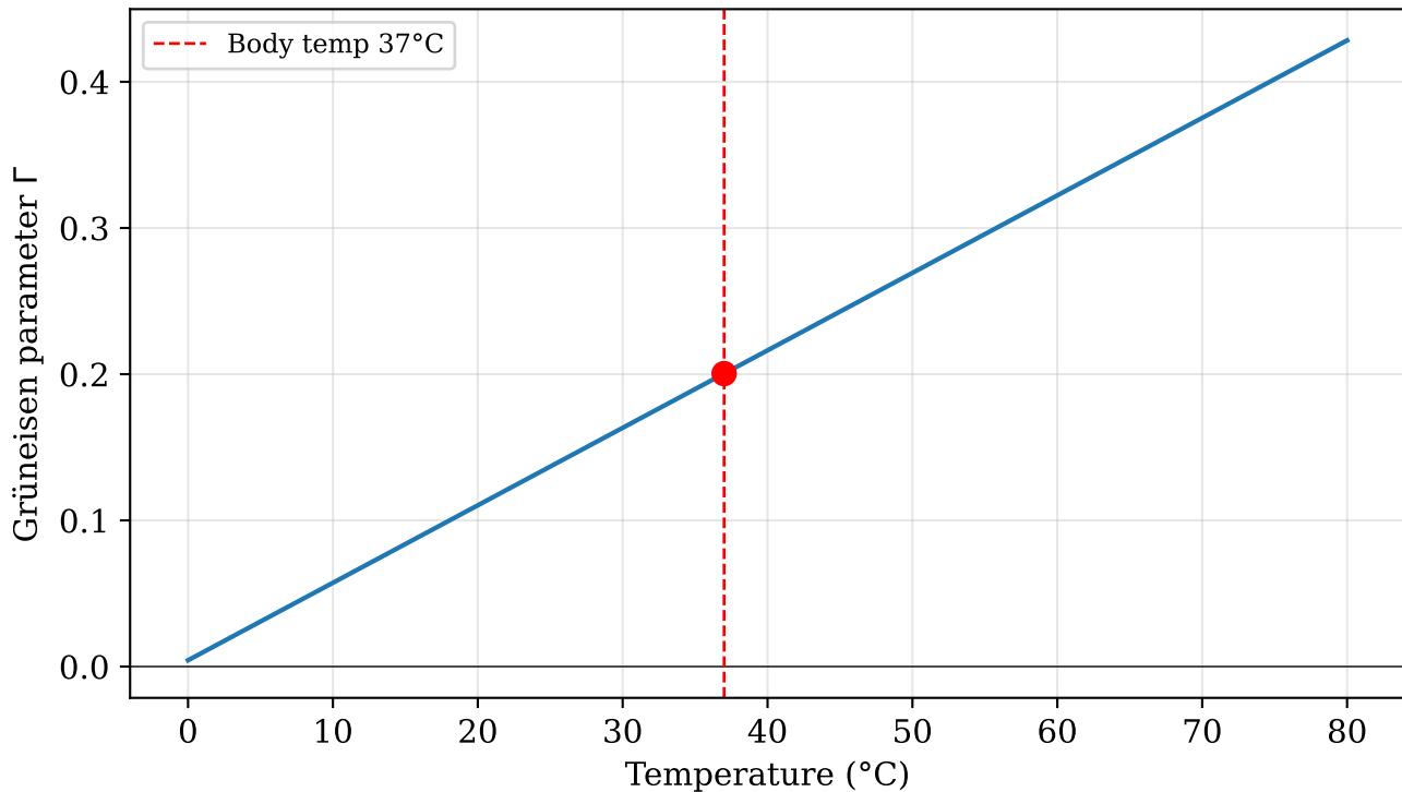
Grüneisen parameter vs temperature (water) \Gamma(T) = 0.0043 + 0.0053 T (Sigrist & Kneubühl 1978)
