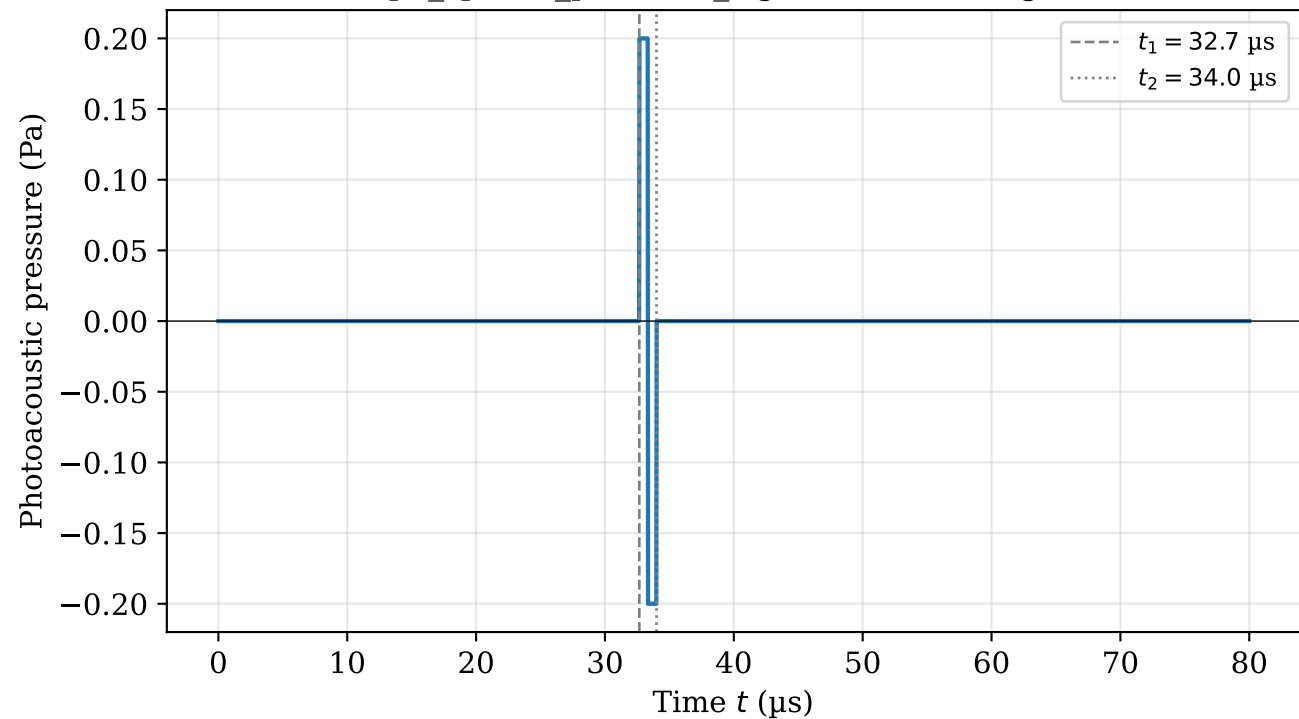
PA signal from spherical absorber ( R = 1.0 mm, r_d = 50 mm) (kw.pa_sphere_pressure_signal, Xu \& Wang 2006)
