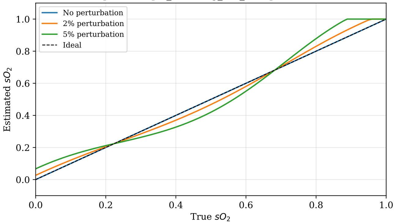
Spectroscopic unmixing: HbO 2 /Hb at 760/850 nm (kw.spectroscopic_unmixing_so2_sweep, Beard 2011)
