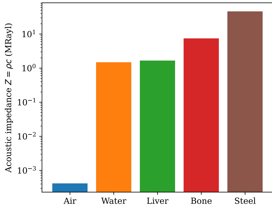
Impedance Z for common media
