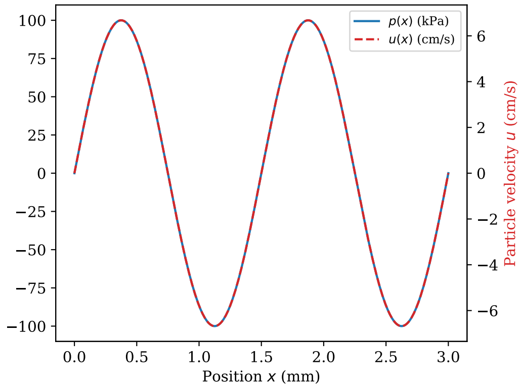
Plane wave: p = \rho c u
