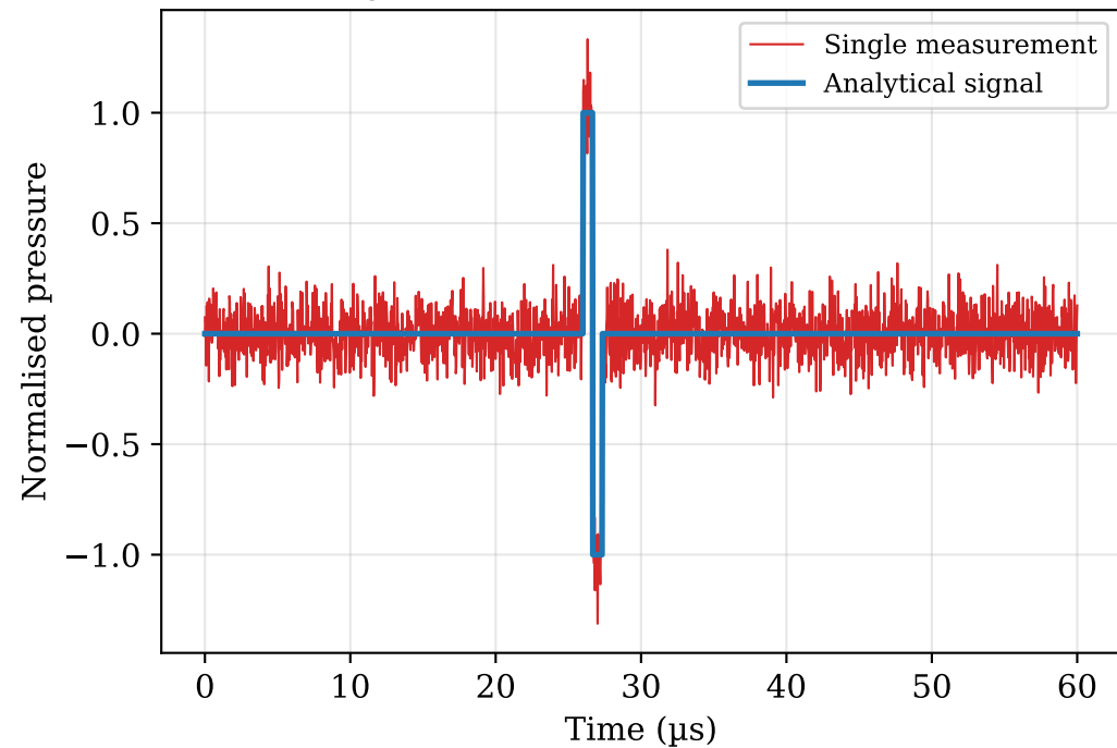
Single PA measurement (SNR \approx 3 dB)
