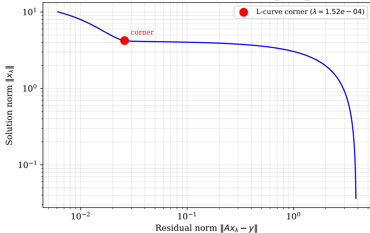
L-curve for Tikhonov regularization (§18.7) 1D Gaussian deconvolution; corner via kw.l_curve_corner
