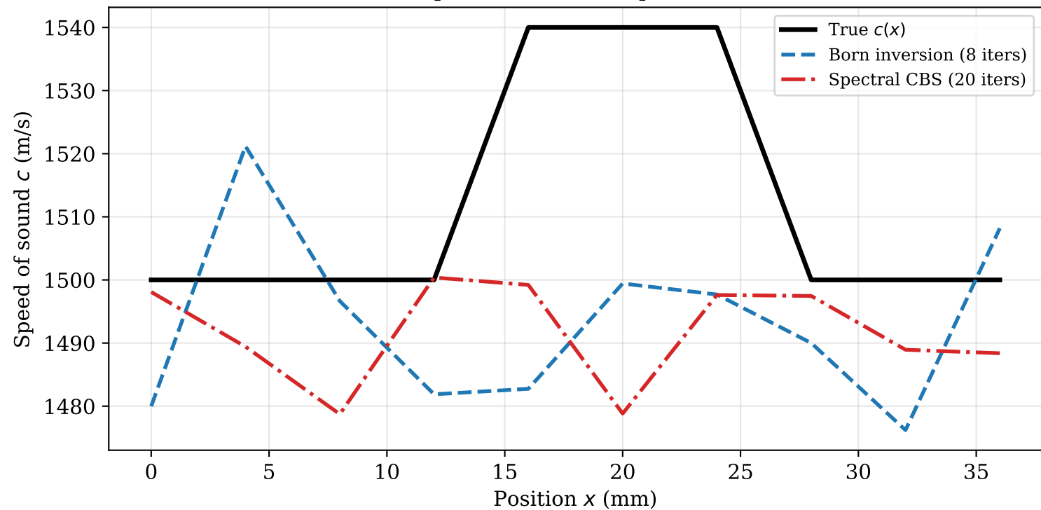
Sound speed reconstruction: Born vs spectral CBS centre-row profile, 10 \times 10 \times 1 phantom, 200 kHz
