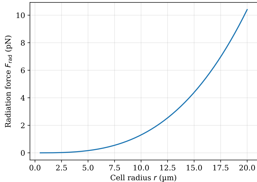
Gor'kov ARF vs cell radius ( P = 50 kPa, f = 1 MHz, f_1 = 0.20 , f_2 = 0.045 )
