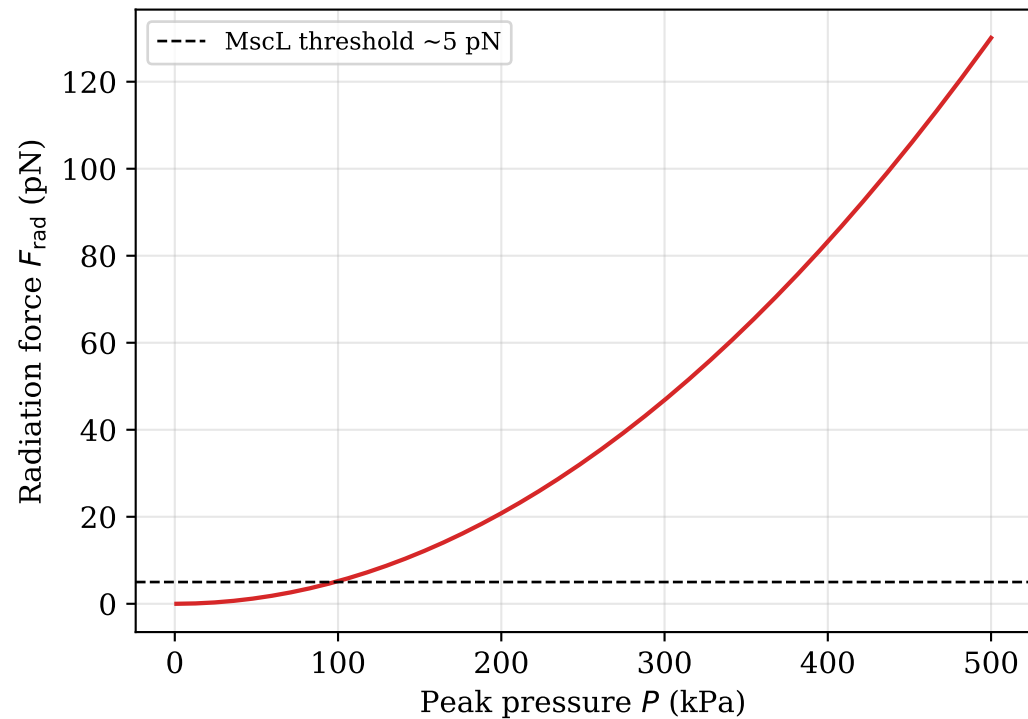
ARF vs pressure ( r = 10 \mu\text{m} )
