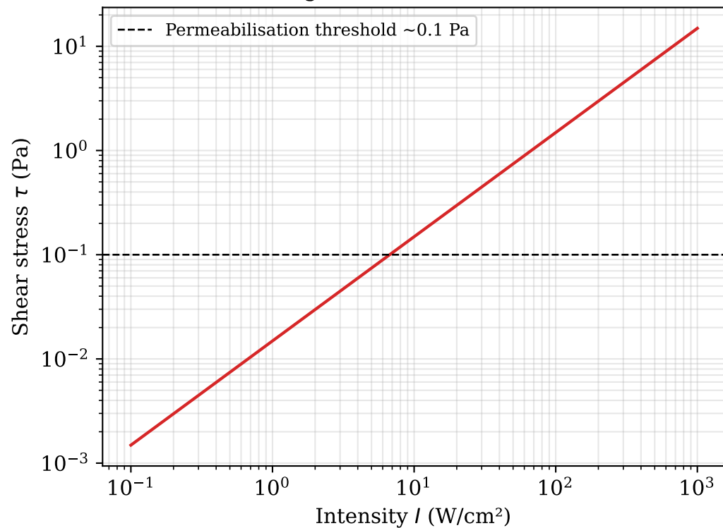
Streaming shear stress on membrane
