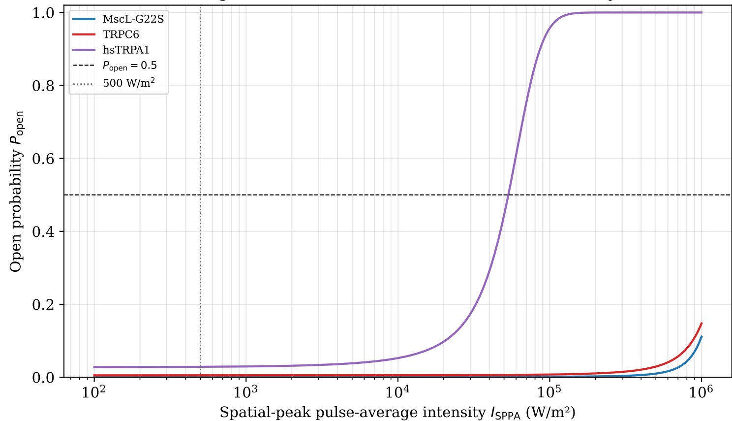
Sonogenetic channel activation vs ultrasound intensity
