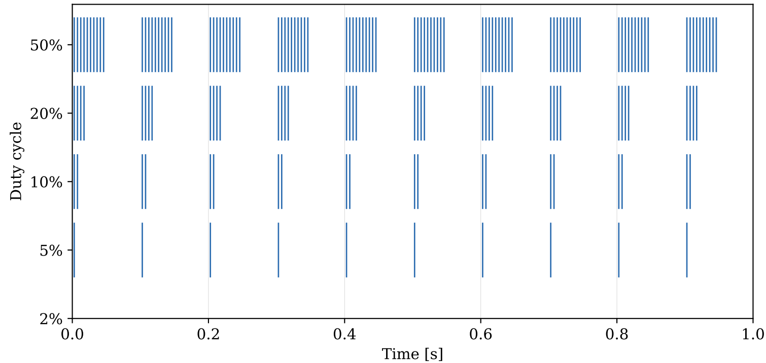
LIF spike raster vs duty cycle (10 Hz PRF, fixed on-current)
