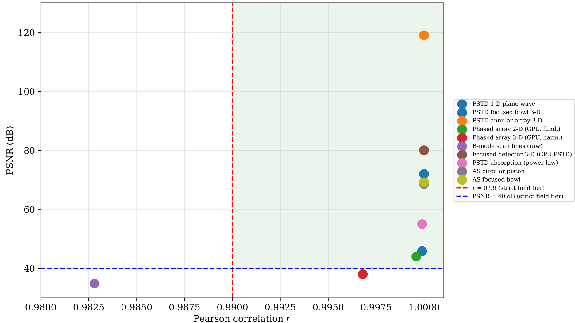
kwavers validation results: closed parity gaps with PSNR
