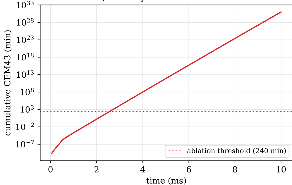
Millisecond, end-of-pulse CEM43 = 9.95e+30 min
