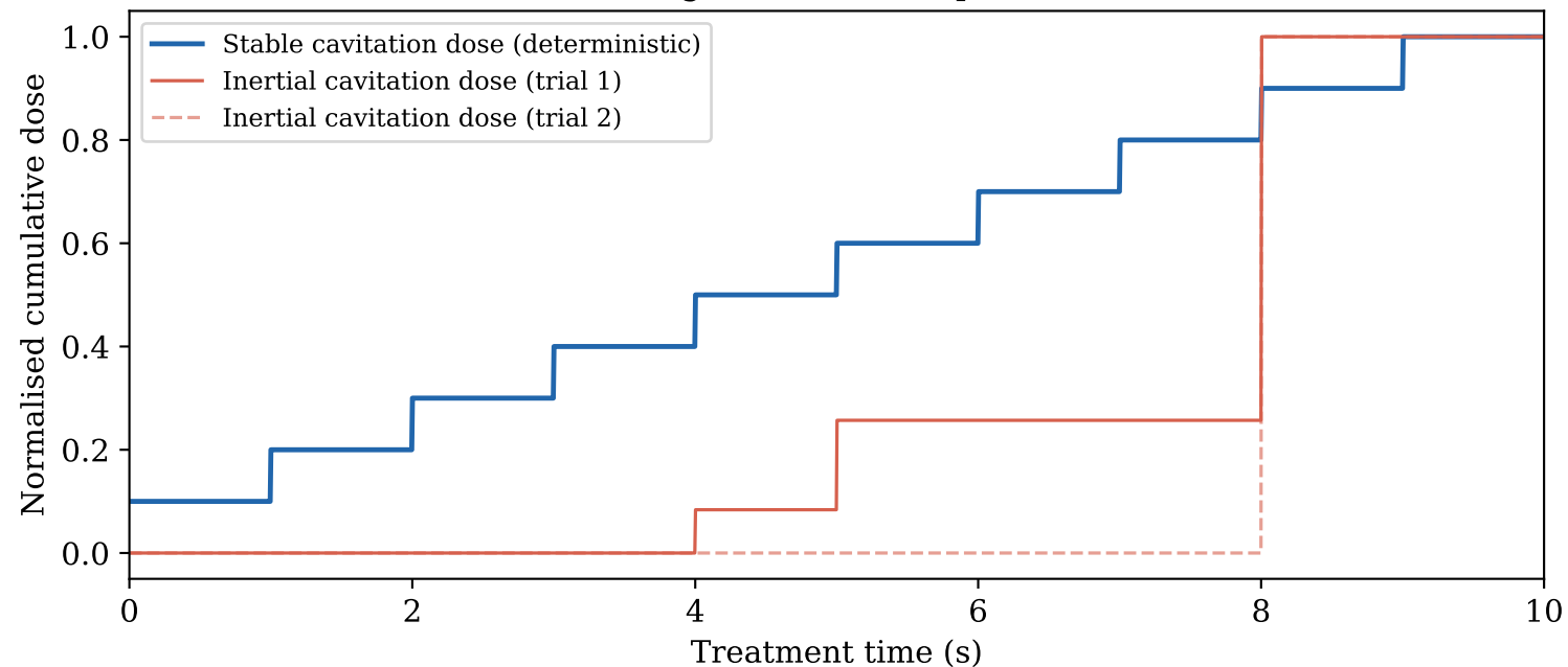
Cavitation dose accumulation SC: deterministic linear growth; IC: compound Poisson (stochastic)
