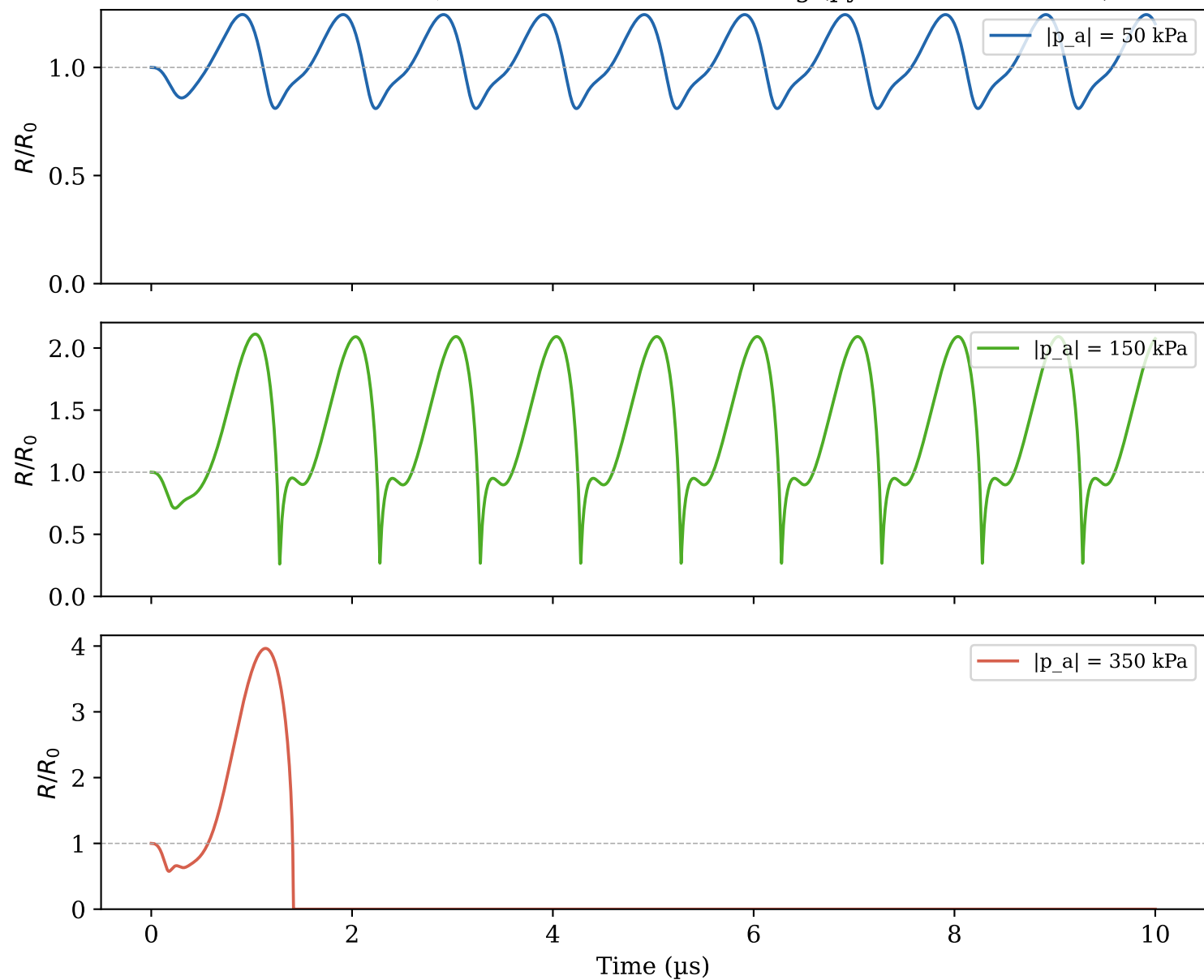
Keller-Miksis MB dynamics — R_0 = 1.5 \text{ }\mu\text{m} , f_0 = 1 \text{ MHz} SonoVue-like shell; LIFU sub-threshold driving (pykwavers Rust RK4)
