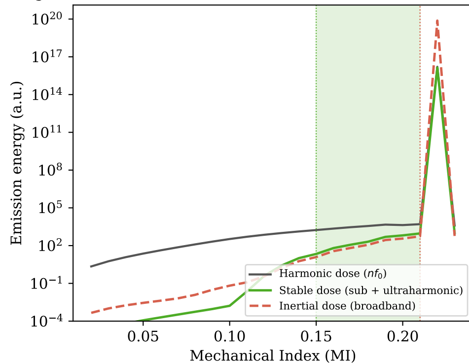
(B) Cavitation dose vs MI green band = stable-cavitation BBB window (MI 0.15–0.21) pressure parks below inertial onset; stable dose accrues
