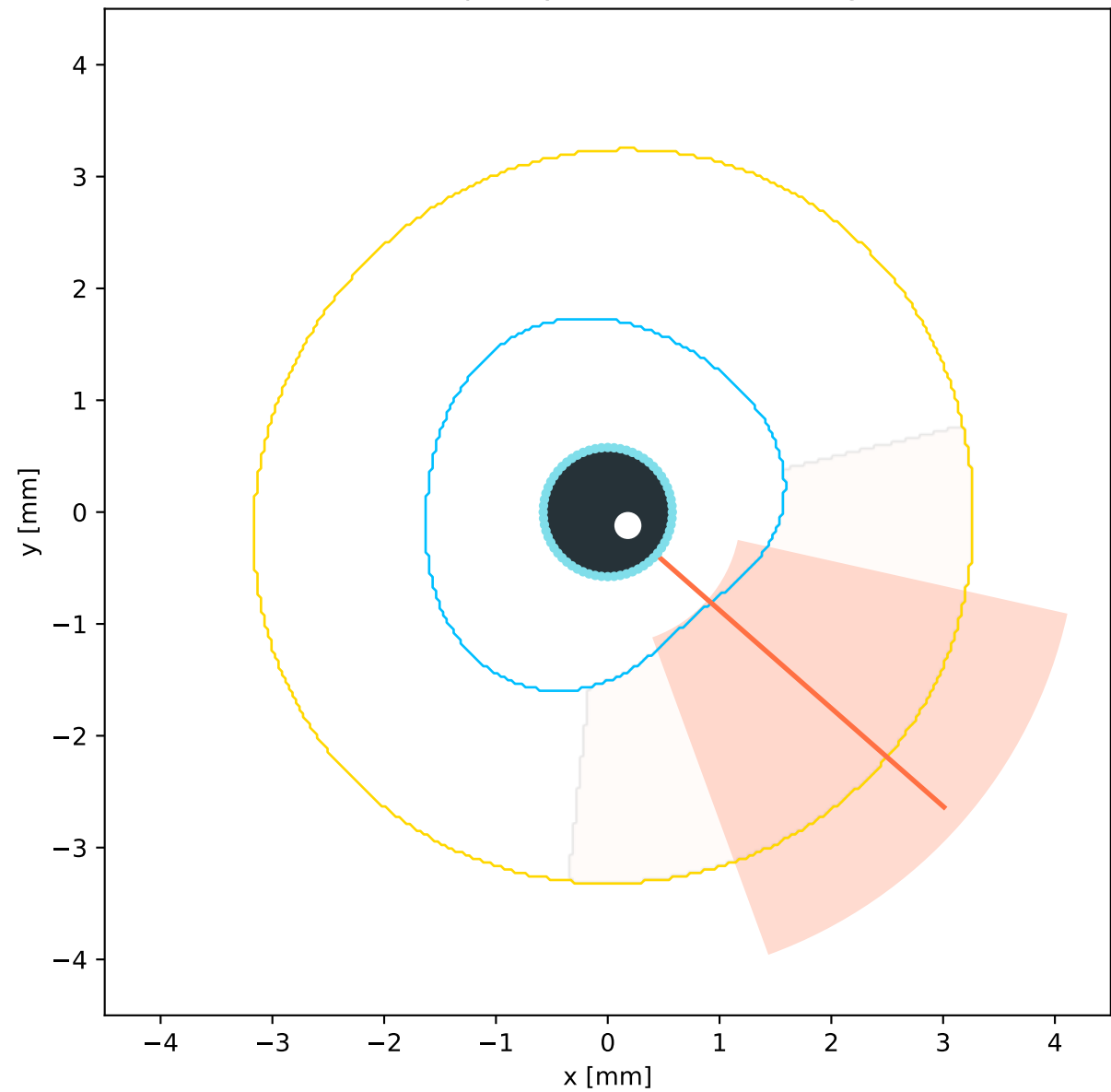
Dual-frequency IVUS catheter design
