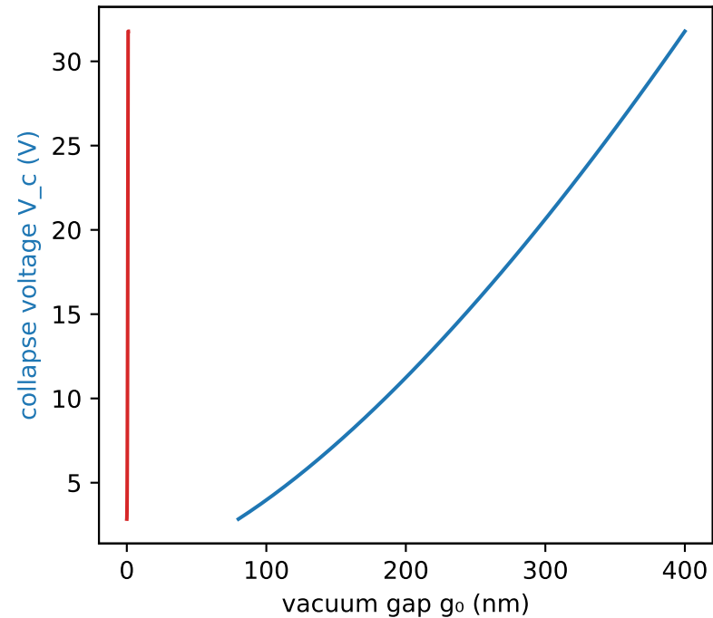
CMUT: collapse voltage ( \propto g^{1.5} ) & bias coupling
