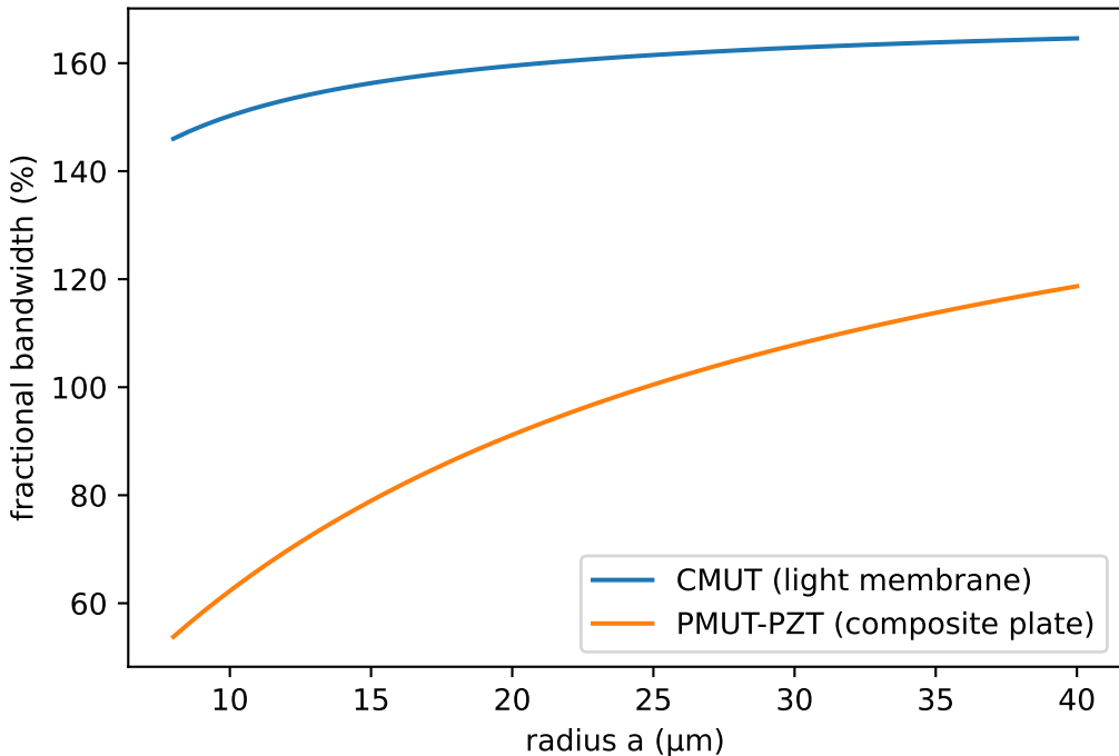
Bandwidth from fluid loading \rightarrow axial resolution
