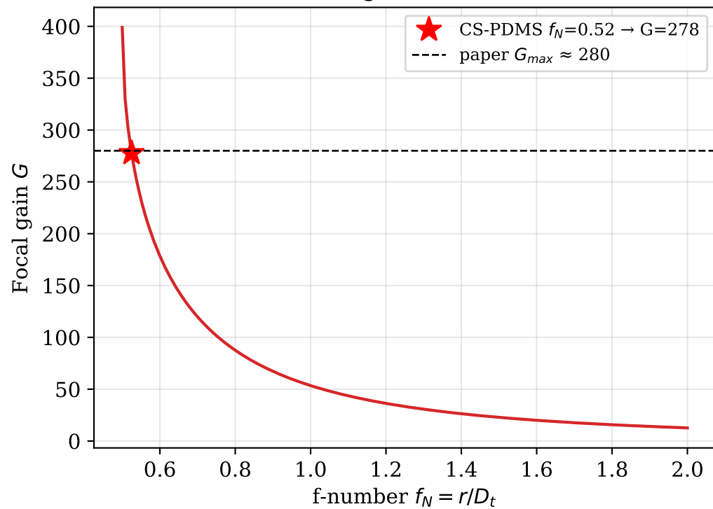
(b) Focal gain vs f-number
