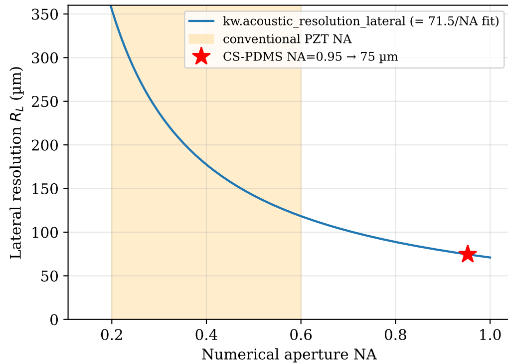
(a) Lateral resolution vs NA (15 MHz)
