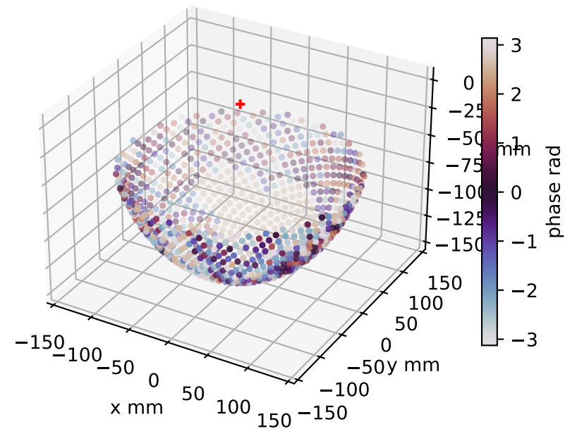
1024-element hemispherical array
