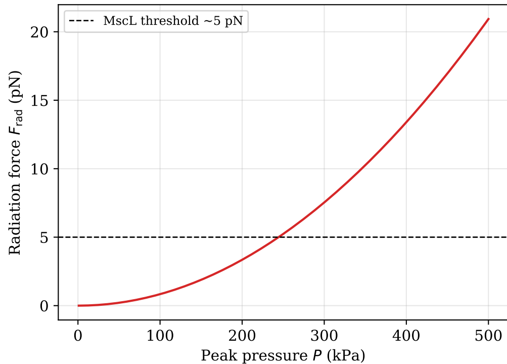
ARF vs pressure ( r = 10 \mu\text{m} )
