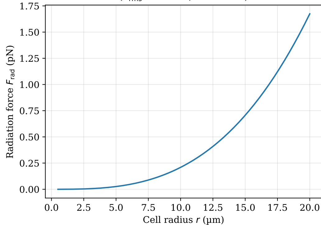
ARF vs cell radius ( P_{\text{rms}} = 50 \text{ kPa} , f = 1 \text{ MHz} )
